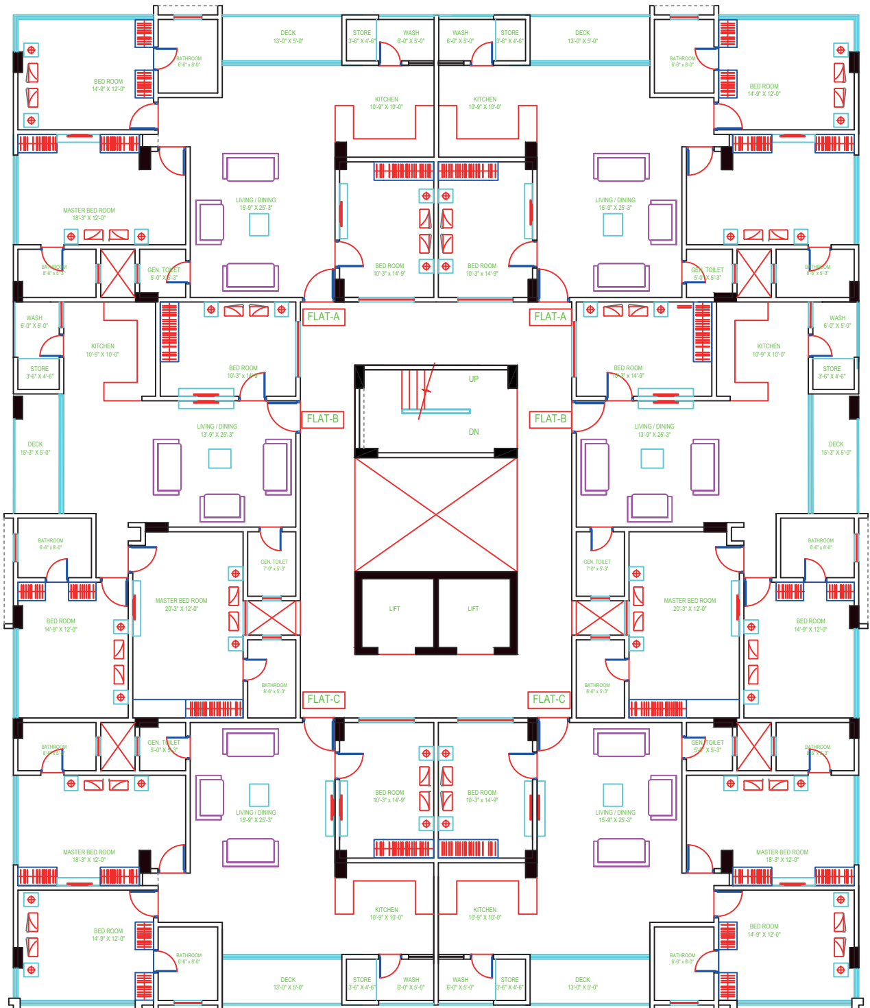
TYPICAL FLOOR PLAN(up to 6th)
